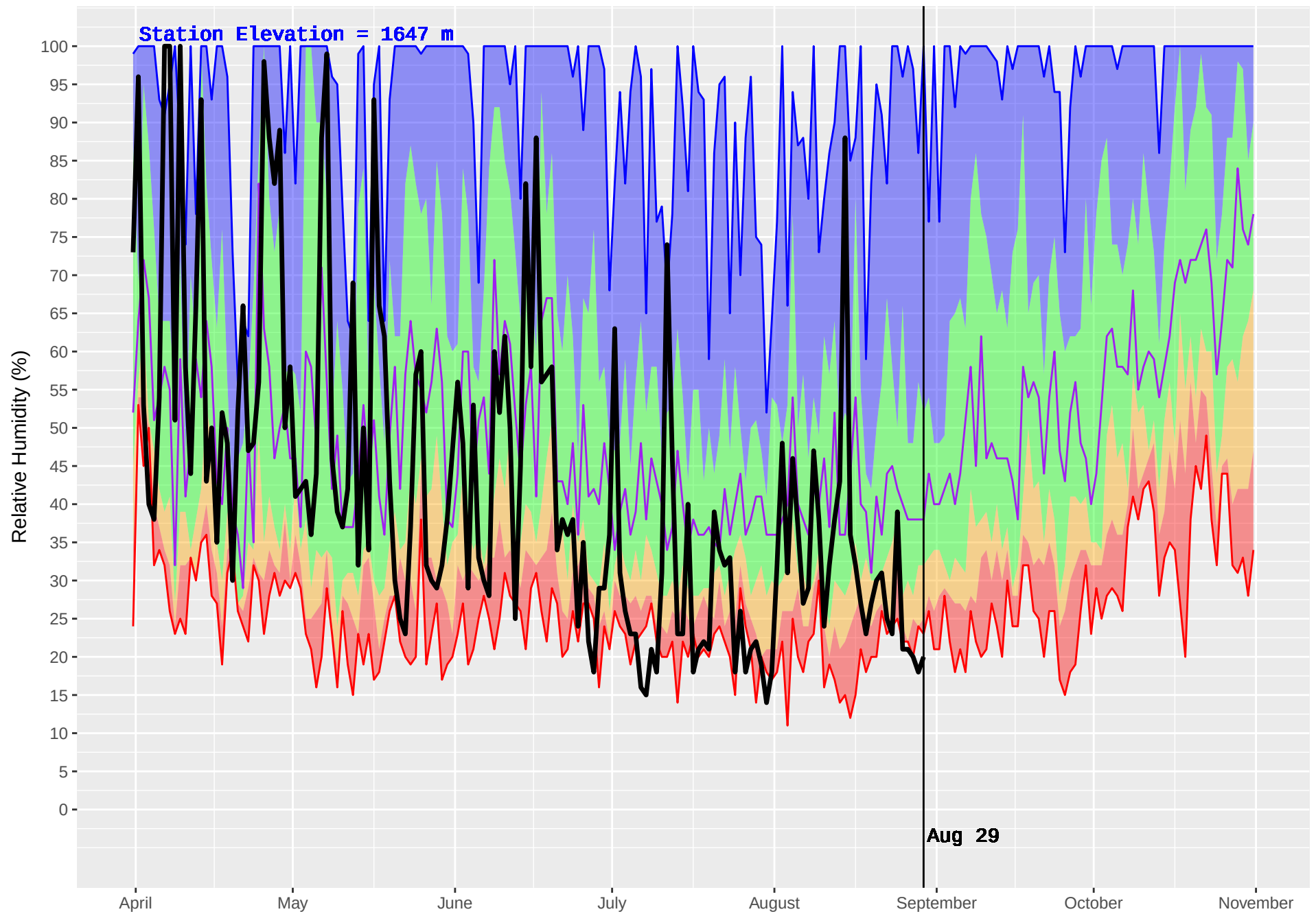
ROUND PRAIRIE (788) : Historical (2001–2016) and Current (2017) Noon Relative Humidity
